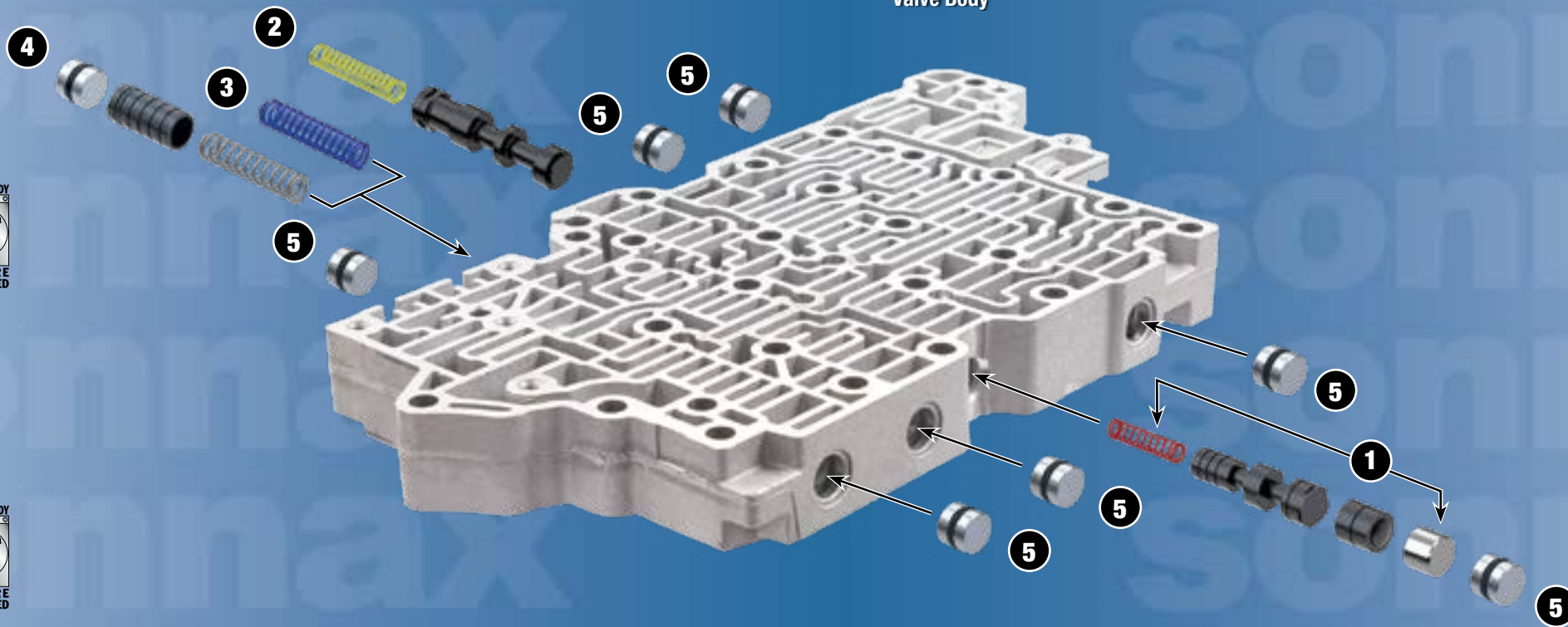
6T70 Upper Valve Body
